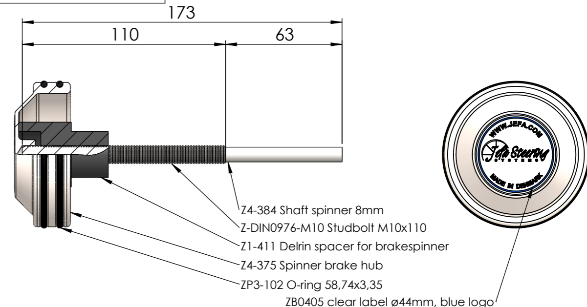
SP-SP173Dis for Jefa diseng. wheel small cone
